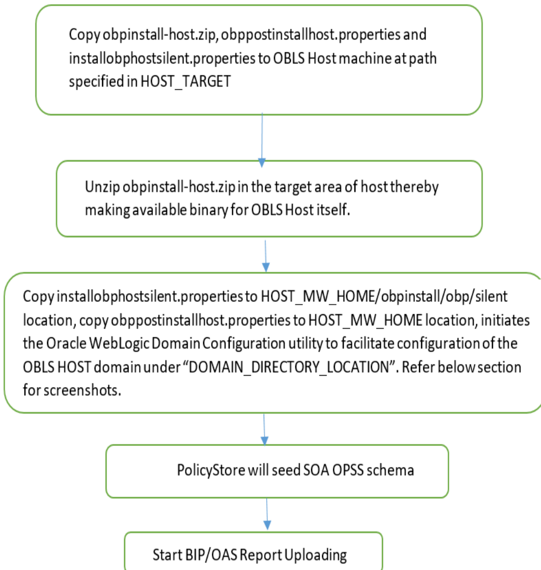
Figure 4–1 Steps in installobphost.sh script
