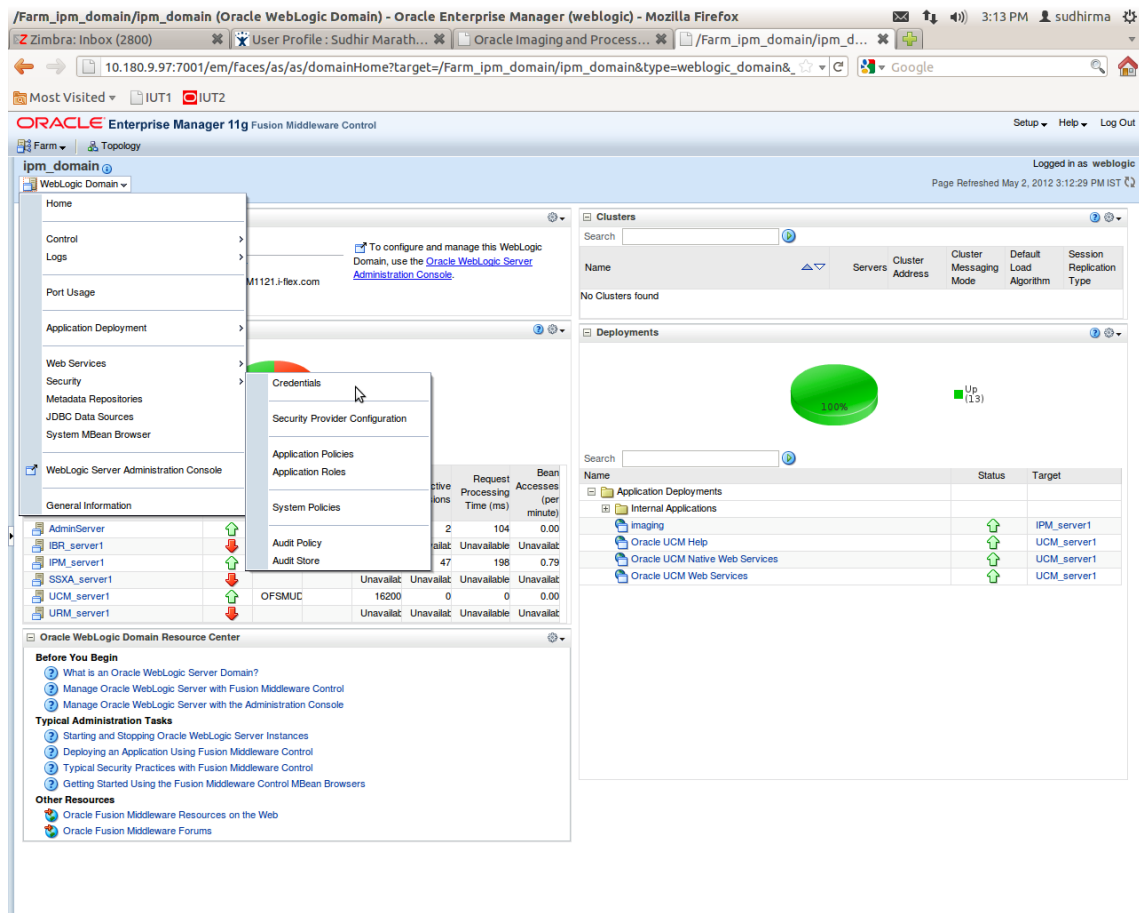
Figure 6–66 Navigate to Weblogic Domain --> Security --> Credentials
