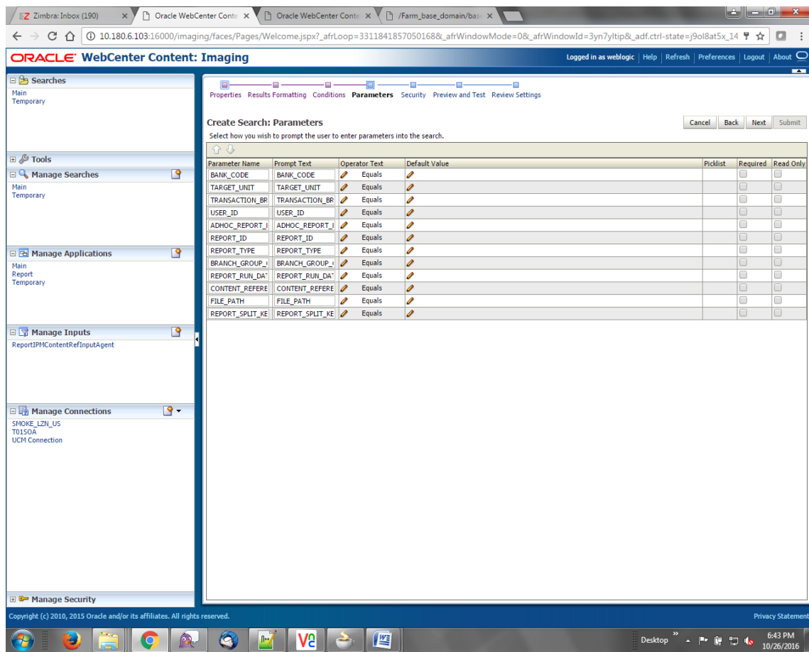
Figure 6–94 Create Search: Parameters
