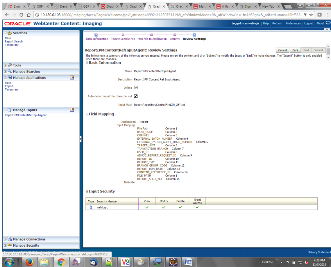
Figure 6–90 Input Agent Details: Review Settings
