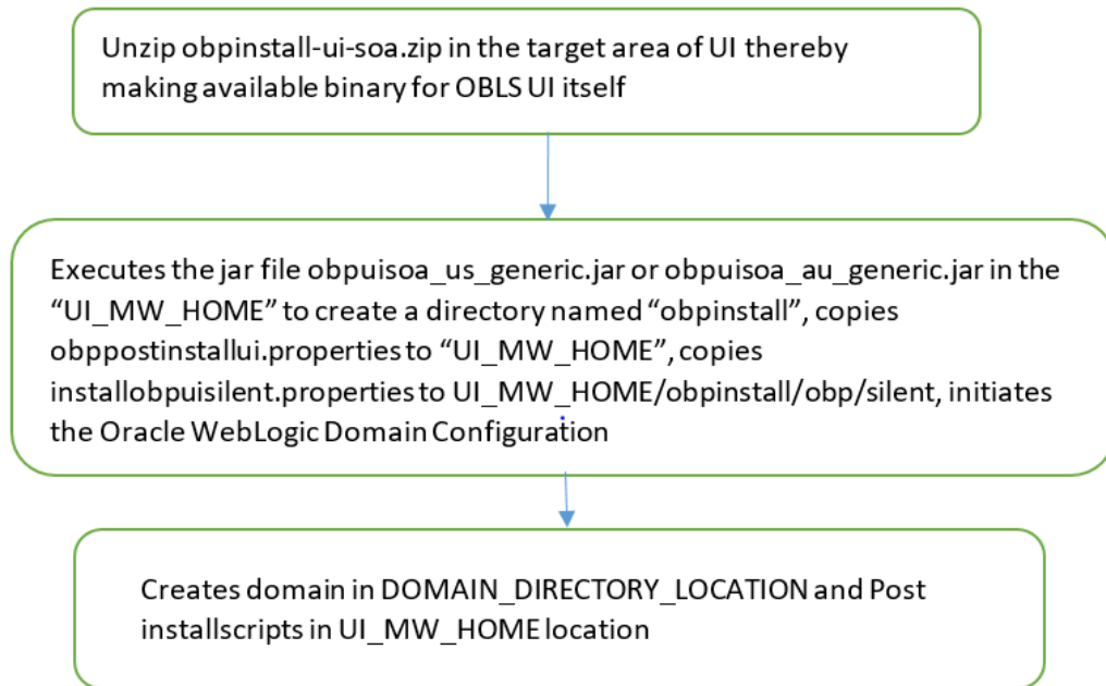
Figure 5–1 Steps in installobpui.sh script
