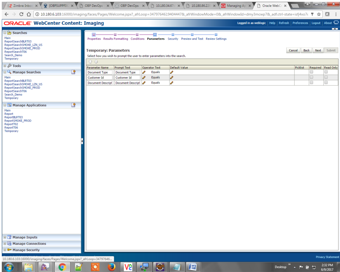
Figure 6–33 Temporary: Parameters
