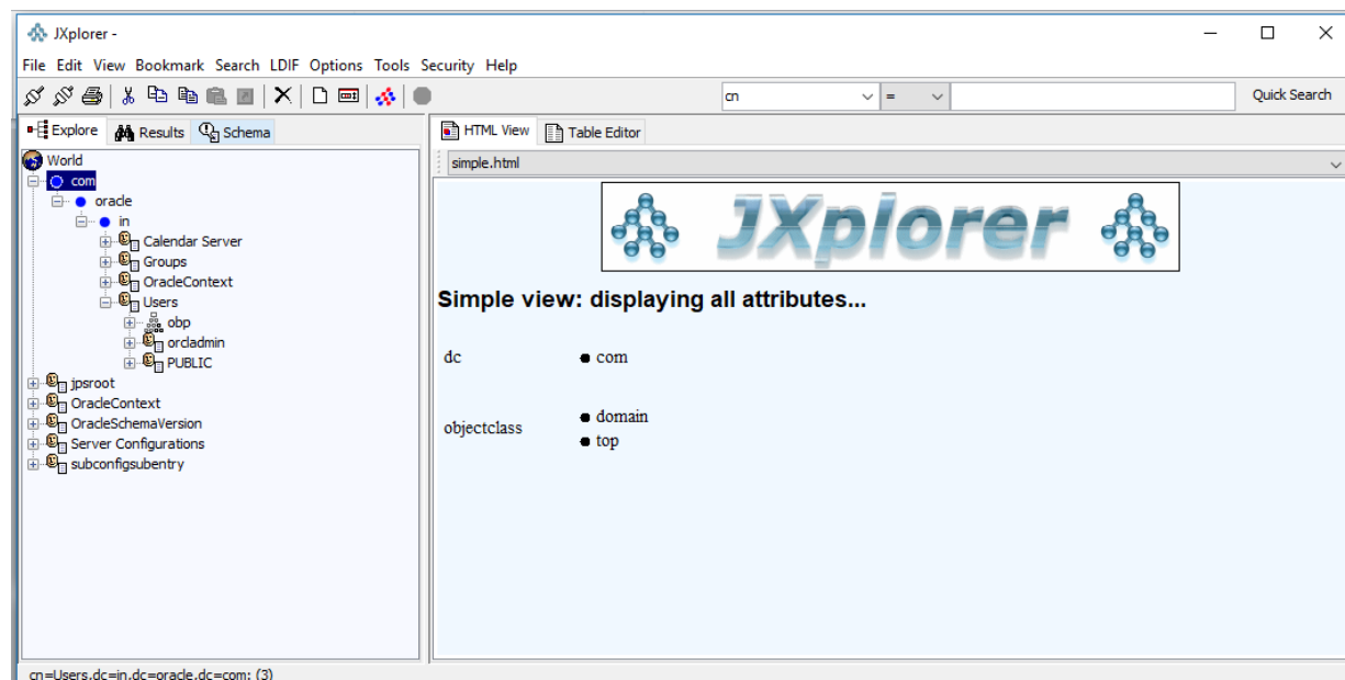
Figure 2–2 JXplorer
