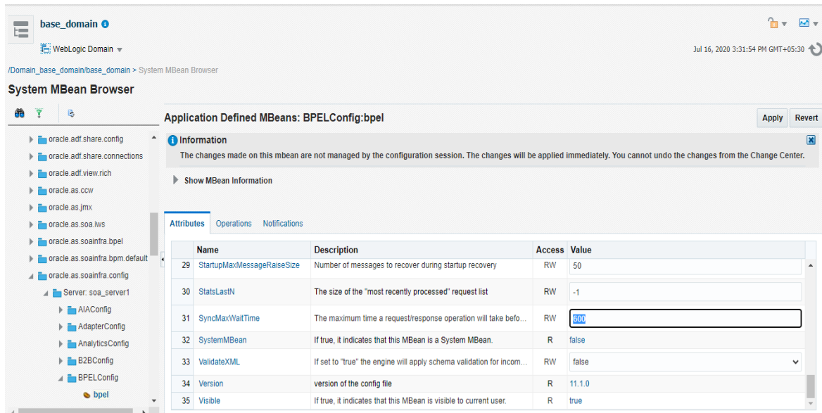
Figure 3–14 BPELConfig:bpeI
