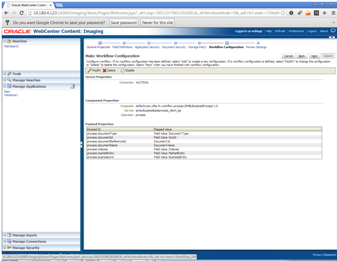
Figure 6–54 Manage Applications - Workflow Configuration
