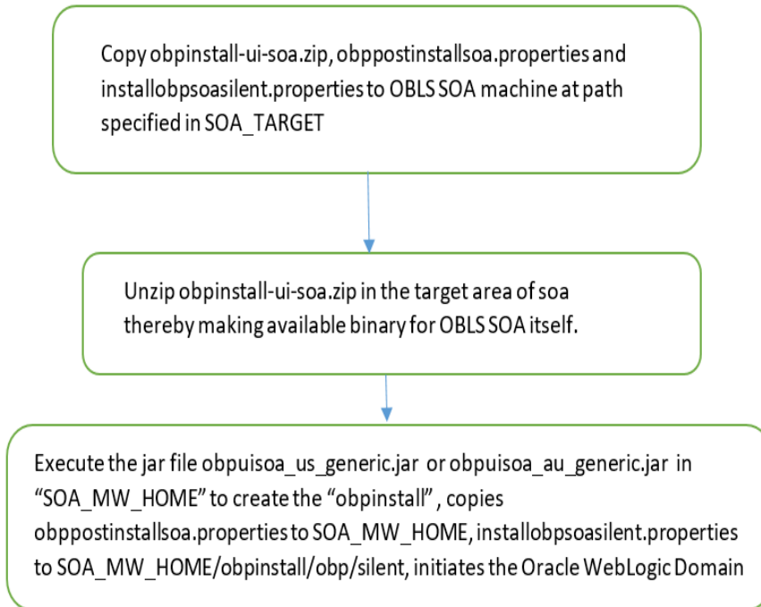
Figure 3–1 Steps in installobpsoa.sh script
